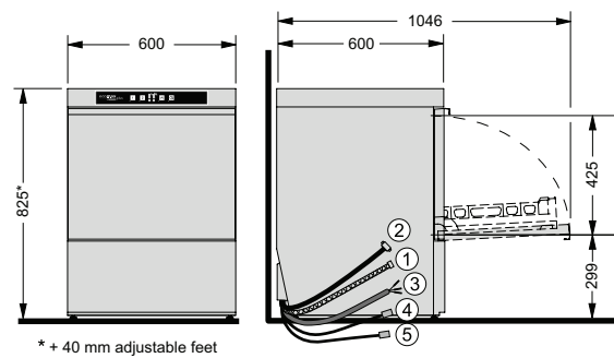
Glasswasher model G503 Undercounter dishwasher model F503
