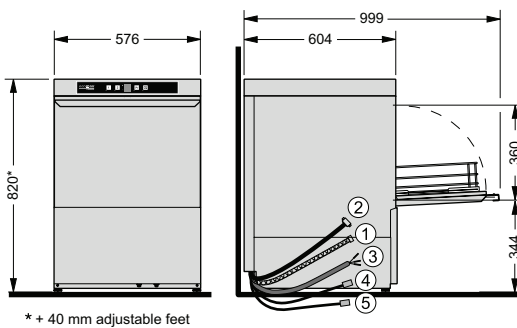
Glasswasher model G504 Undercounter dishwasher model F504
