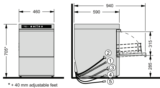
Glasswasher model G403
