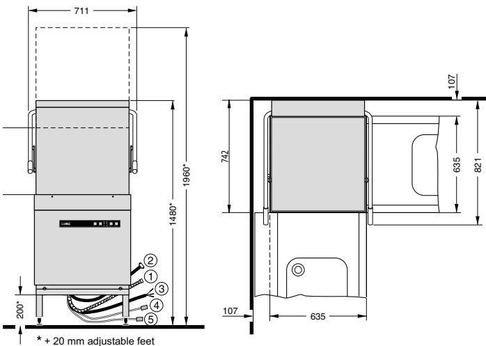
Hood-type dishwasher model H602
