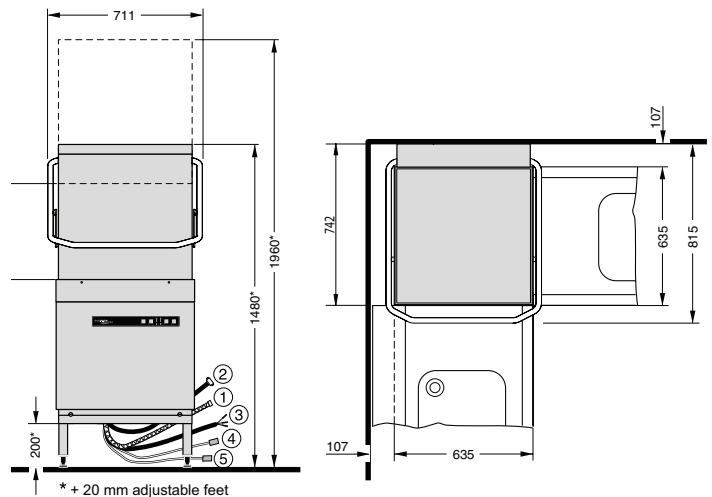
Hood-type dishwasher model H603
