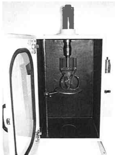
Figure C.1 Soundproof Box
