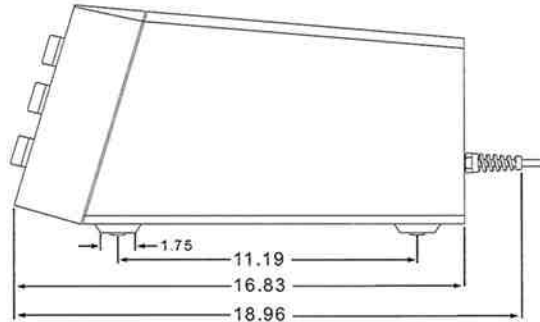
Figure 2.3 250/450 Sonifier Side View Dimensions
