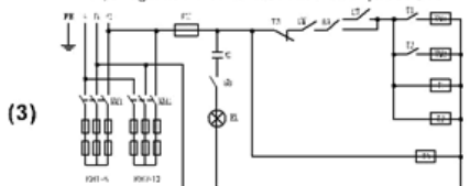
Wiring diagram for 380V series oven.
